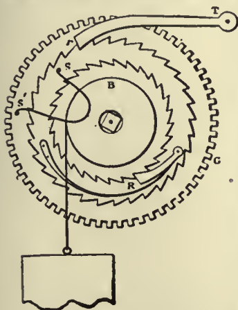
FIG. 25.—Harrison's Going-Ratchet.
